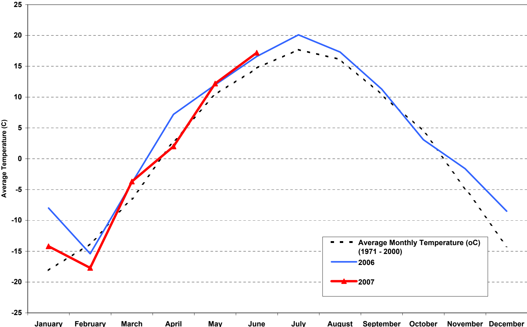
Average monthly temperature at Atikokan vs. 1971 - 2000 average
