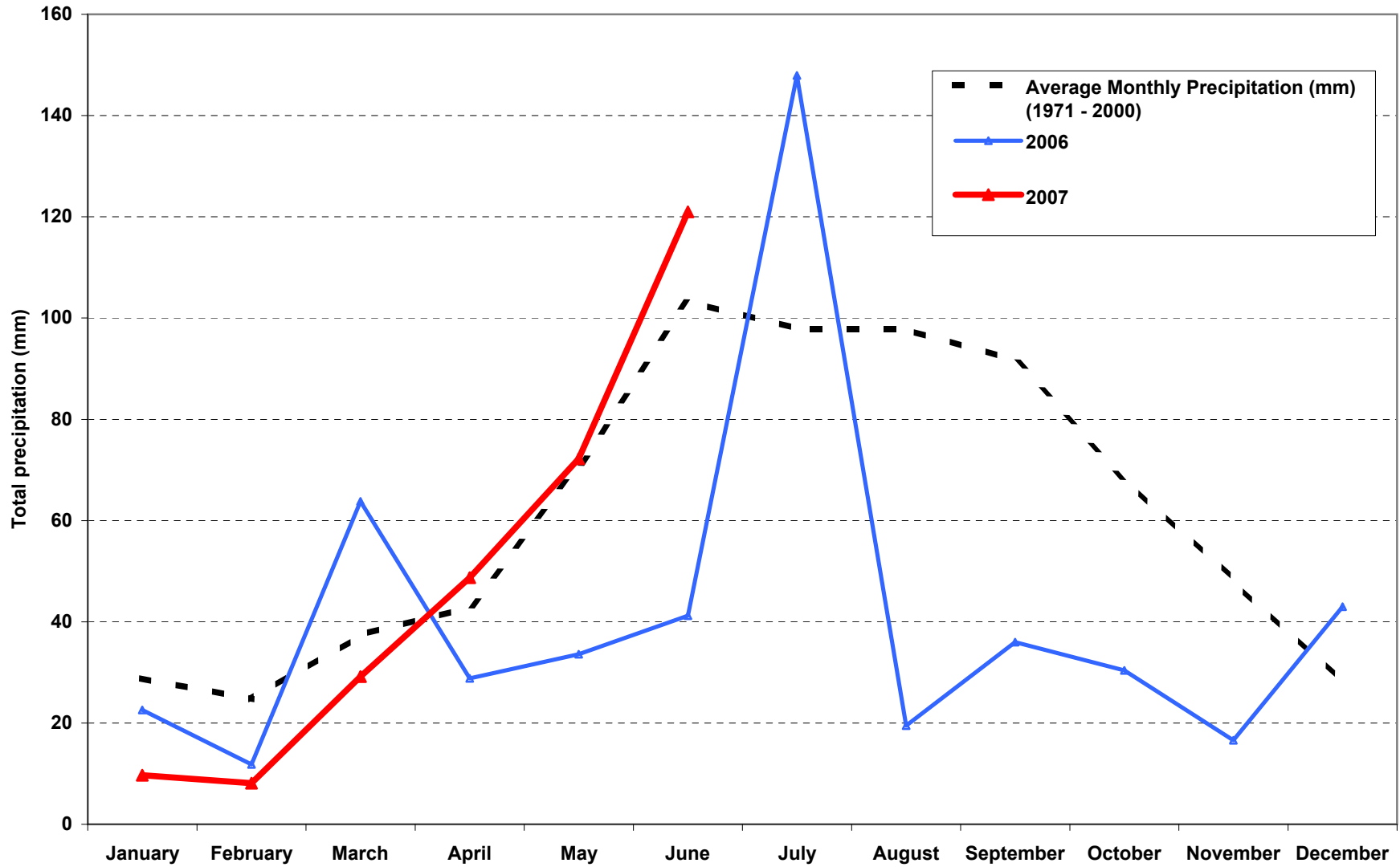
Total monthly precipitation at Atikokan vs. 1971 - 2000 average
